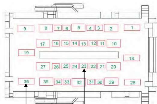
View of Front Face of BCM Connector 3
