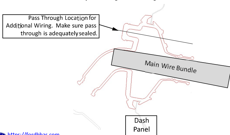
Detail A - Section Through Dash Wiring Grommet
